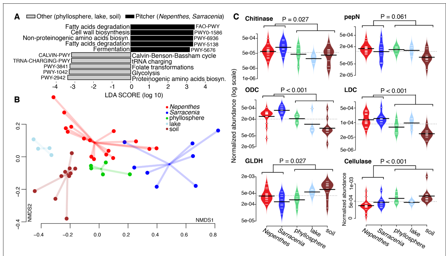
Figure 5. Pitcher plant microbiomes are enriched in degradation genes. (A) Gene pathways enriched in pitcher plant versus other environmental metagenomes. (B) NMDS plot of functional gene families comparing pitcher plant and environmental metagenomes. (C) Relative abundance of gene families in metagenomes. Abbreviations: pepN = aminopeptidase N; ODC = ornithine decarboxylase; LDC = lysine decarboxylase; and GLDH = glutamate dehydrogenase.
