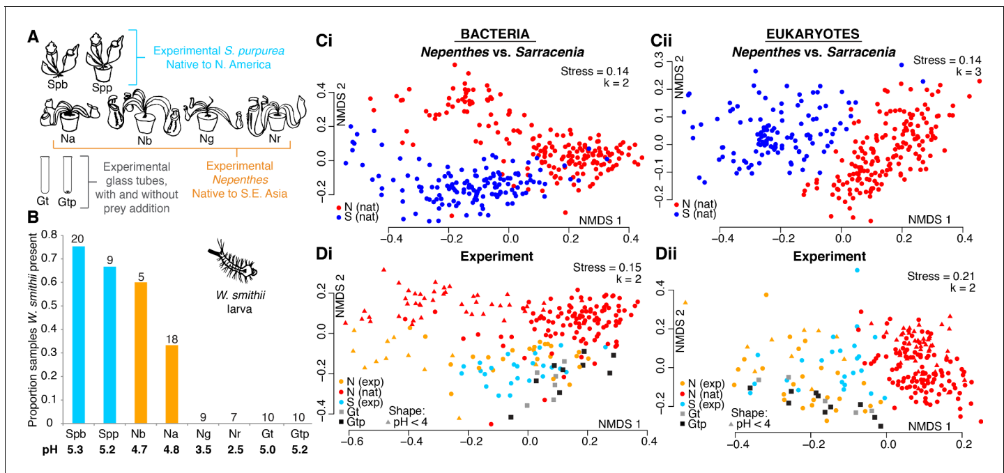
Figure 4. A manipulative field experiment demonstrates that Nepenthes pitchers in a Sarracenia habitat assemble Sarracenia -like microcosms. (A) Experimental treatments: Spb = Sarracenia purpurea bog; Spp = S. purpurea pot; Na = Nepenthes ampullaria ; Nb = N. bicalcarata ; Ng = N. gracilis ; Nr = N. rafflesiana ; Gt = glass tube; Gtp = glass tube with sterilized prey. (B) Wyeomyia smithii (pitcher plant mosquito) larvae colonized their native S. purpurea hosts, as well as foreign Nepenthes species with average pH > 4, but not pitcher-shaped glass tubes. Numbers of samples are listed above each category, and average pH values are listed below. (C) Natural microcosms of Nepenthes and Sarracenia pitchers sampled in SE Asia or North America house different organisms (Ci and Cii). (D) However, experimentally-relocated Nepenthes converge on Sarracenia -like communities and differ from those of natural Nepenthes (Di and Dii), except for bacterial communities sampled from Nepenthes in which pH < 4 (Di). Glass tubes (with or without added prey) of a pitcher-like form assemble communities that are similar to those of experimental pitchers (Di and Dii).
