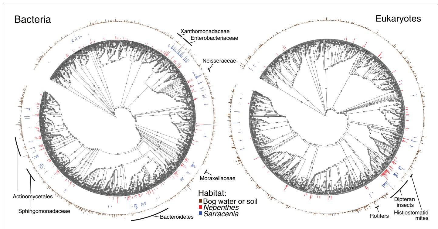
Figure 2. Nepenthes and Sarracenia pitchers are colonized by related organisms. Phylogeny of bacterial and eukaryotic OTUs found in soil and bog samples (brown); and OTUs present in at least 10% of field collected Nepenthes (red) or Sarracenia (blue) samples. The height of the colored bars surrounding each tree corresponds to the natural log of the relative abundance of reads from each OTU, normalized across the samples in each category. Labels designate monophyletic clades where high proportions of OTUs are shared between Nepenthes and Sarracenia samples. Gray dots mark branches leading to nodes with bootstrap support of 0.7 or higher. The bacterial tree is rooted in Archaea and the eukaryotic tree is rooted in Streptophyta.
