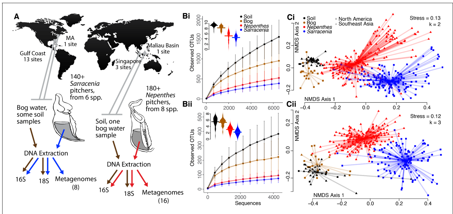
Figure 1. Pitcher microcosms are more similar to each other than they are to communities of surrounding habitats. (A) Geography of sampled Sarracenia and Nepenthes and experimental approach. (B) The species richness (displayed as rarefaction plots) and Shannon diversity (inset beanplots) of both bacterial (i, top) and eukaryotic (ii, bottom) communities was lower in pitchers than in surrounding soil and bog water. Error bars are standard deviations. (C) Community composition using the unweighted UniFrac metric for bacteria (i, top) and eukaryotes (ii, bottom). NMDS stress and dimensions (k) are listed, and the center of each cluster is the category's median value.
