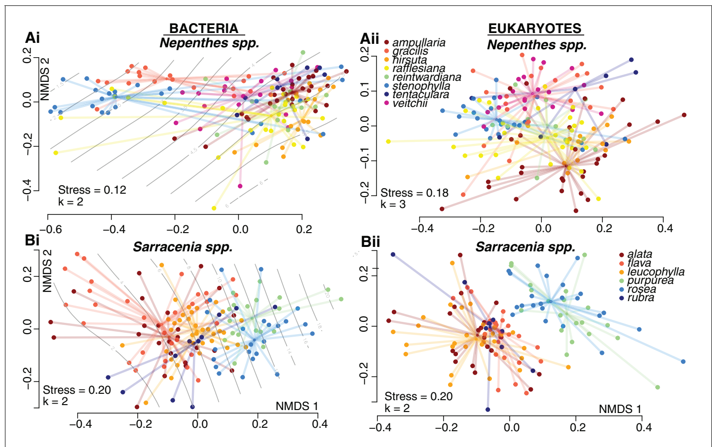
Figure 3. Community compositions differ by host species within both Nepenthes and Sarracenia pitchers. NMDS ordinations of pitcher samples, colored by host species. Ordisurf vectors with correlations greater than 0.3 are mapped onto the ordinations: pH in (Ai) and volume in (Bi).
