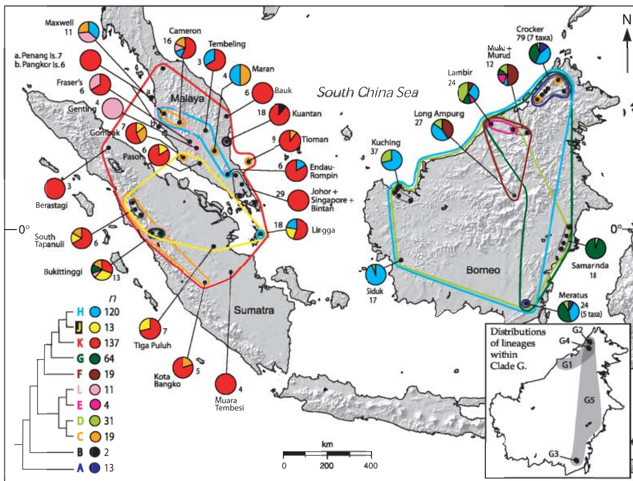
Fig. 3 Approximate distributional ranges of Decacrema lineages (coloured lines) as inferred by sampling locations. Pie charts show inferred lineage composition of locations (proportional to abundance as sampled), with sample sizes indicated. Pie charts and distribution lines are colour-referenced to the ant phylogeny at bottom left. Clades Cb and Cms (C in Borneo and Malaya + Sumatra, respectively), and Gs (in Sumatra), G1, G2, G3, G4 and G5 are not detailed in the phylogeny (see Fig. 1 for detail).
