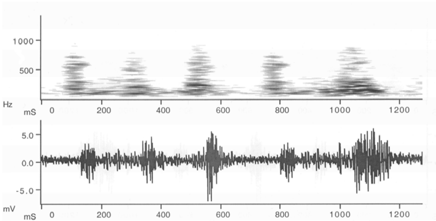
Fig. 2. Waveform (bottom) and spectrogram (top) of a pulse train produced by a E. elvina caterpillar.
