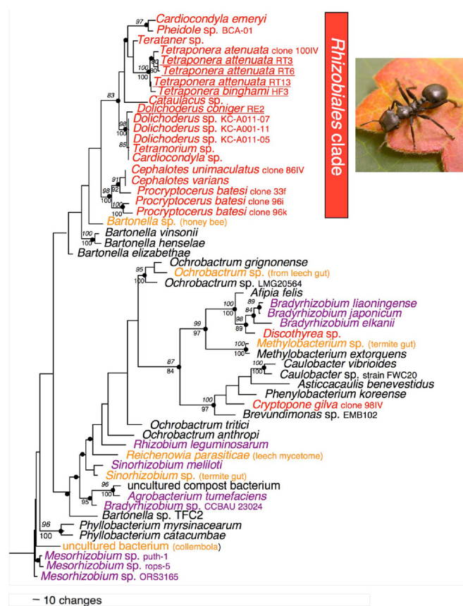
Fig. 1. 16S rRNA phylogeny of ant-associated Rhizobiales symbionts and their GenBank relatives. Tree topology was obtained through a maximum-likelihood analysis, and statistical support from each of three separate analyses is indicated at each node: Bootstrap values for nodes with \geq 80\% support are indicated above (likelihood) and below (parsimony) the branches leading to their respective nodes; posterior probabilities \geq 90\% from Bayesian analyses are similarly indicated using black circles. Ant-associates are presented in red font and named after their hosts; those identified in previous studies are presented with underlined font. In several instances, collection or clone IDs are included to help distinguish between similarly named associates. Bacteria from plants and other animals are presented in purple and orange fonts, respectively, whereas those from other or unspecified habitats are in black. GenBank accession numbers and full sequence names for taxa in this tree are presented in Table S6. Photo inset by C. S. Moreau. Outgroups Wolbachia and P. aeruginosa are not pictured.
