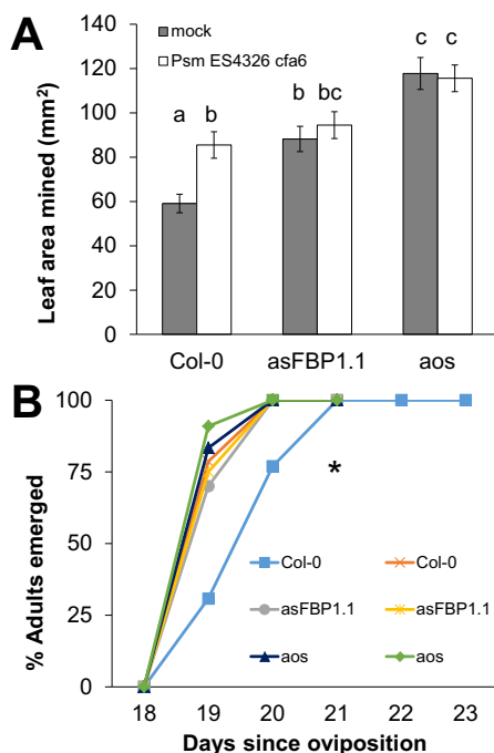
Fig. 4. Enhanced consumption of leaf material and accelerated development of S. flava larvae in P. syringae -infected leaves are not found in the asFBP1.1 and aos mutants of Arabidopsis. (A) Mean leaf area mined (LAM) by S. flava larvae reared in wild-type (WT; Col-0) and mutant Arabidopsis leaves pre-infected with Psm ES4326 cfa6 compared to LAM by larvae reared in mock-inoculated leaves. Larvae were transferred from WT nursing plants in the second instar into the experimental plants and allowed to feed for 48 hours. Error bars represent standard error of the mean. (B) Percentage of S. flava pupae having eclosed as adults over time shown in days after the day of oviposition in the nursing plants. Letters in (A) indicate statistically significant differences (two-way ANOVA with post hoc Tukey's HSD tests, P < 0.05 ). The asterisk in (B) indicates a statistically significant difference between mock-inoculated Col-0 WT plants and the other treatment groups ( \chi^2 tests, P < 0.05 ). N = 15 –20 plants per treatment group.
