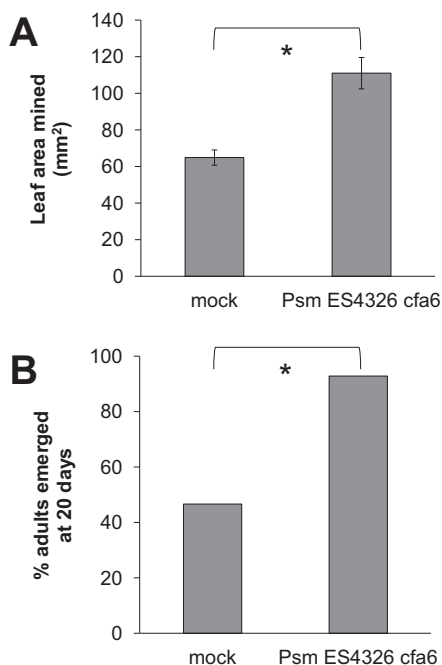
Fig. 2. Saptomyza flava larvae consume more and develop faster in P. syringae -infected leaves. (A) Mean leaf area mined (LAM) by S. flava larvae reared in wild-type (WT; Col-0) Arabidopsis leaves pre-infected with Psm ES4326 cfa6 compared to LAM by larvae reared in mock-inoculated leaves. Larvae were transferred from WT nursing plants in the second instar into the experimental plants and allowed to feed for 48 hours. (B) Percentage of S. flava pupae having eclosed as adults at 20 days after the day of oviposition in the nurse plants. Error bars represent standard error of the mean. Asterisks indicate a statistically significant difference (two-tailed Student's t -test, P < 0.05 in (A); \chi^2 test, P < 0.05 in (B)) between treatments ( N = 15 –20 plants per treatment).
